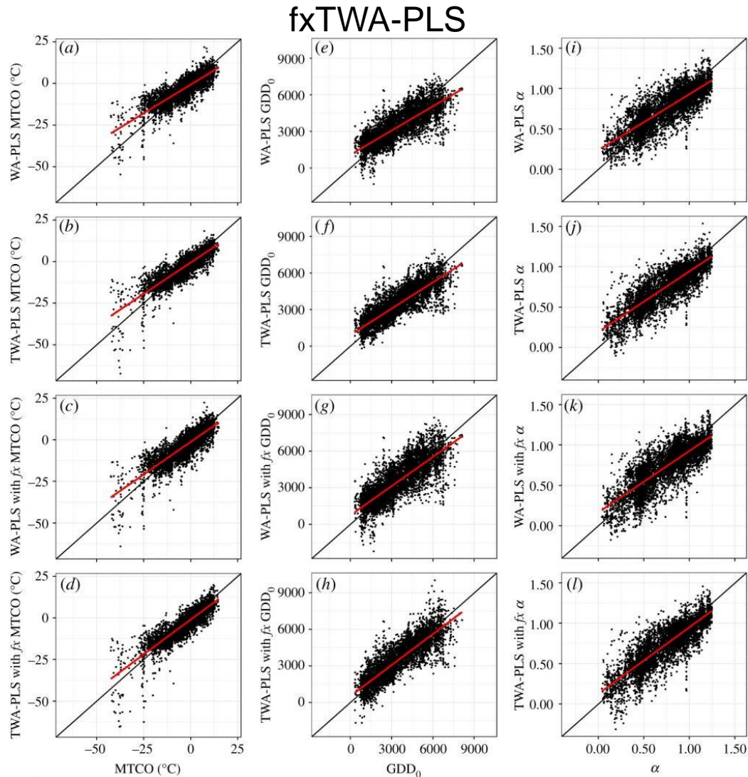
Figure 2. Reconstructed modern climates vs observed modern climates. (Liu et al., 2020)
